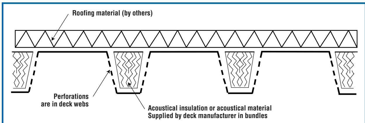
Figure 1: 1-1/2" and 3" acoustic roof deck
