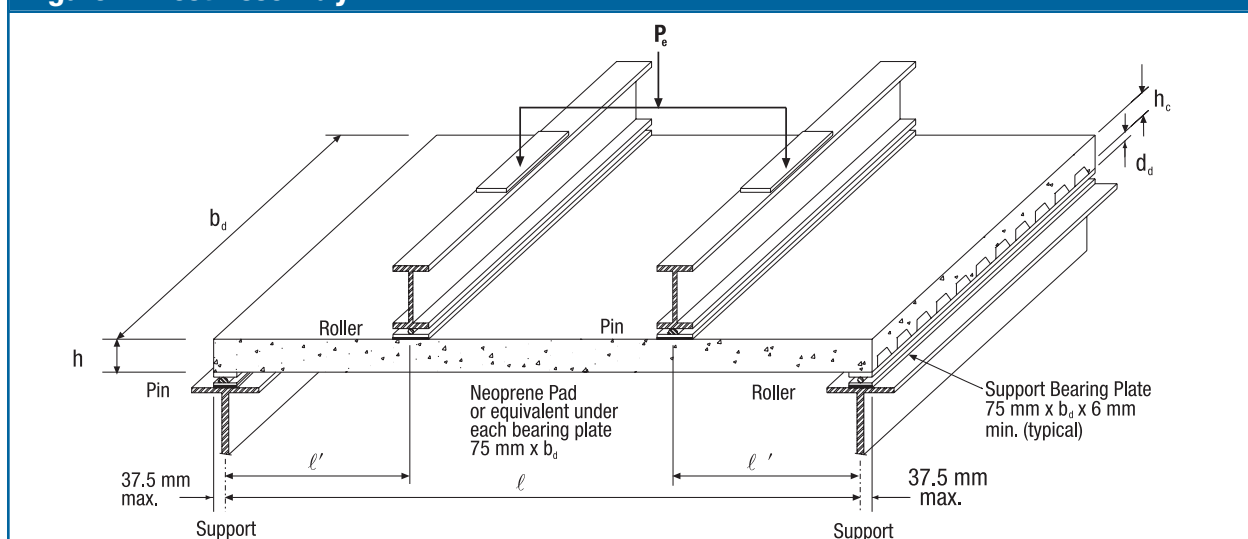
Figure 1: Test Assembly
